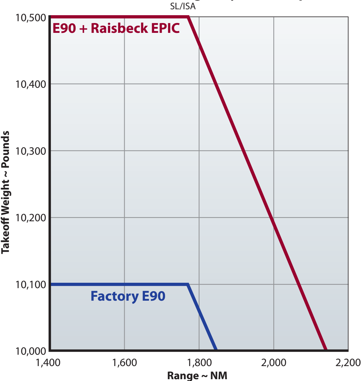
E90 Series EPIC Takeoff Range/Payload Comparison
